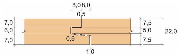
Fig. 1 VMG Lignum Board- T&G4 Board, 22°mm. Tongue and groove profiles.
